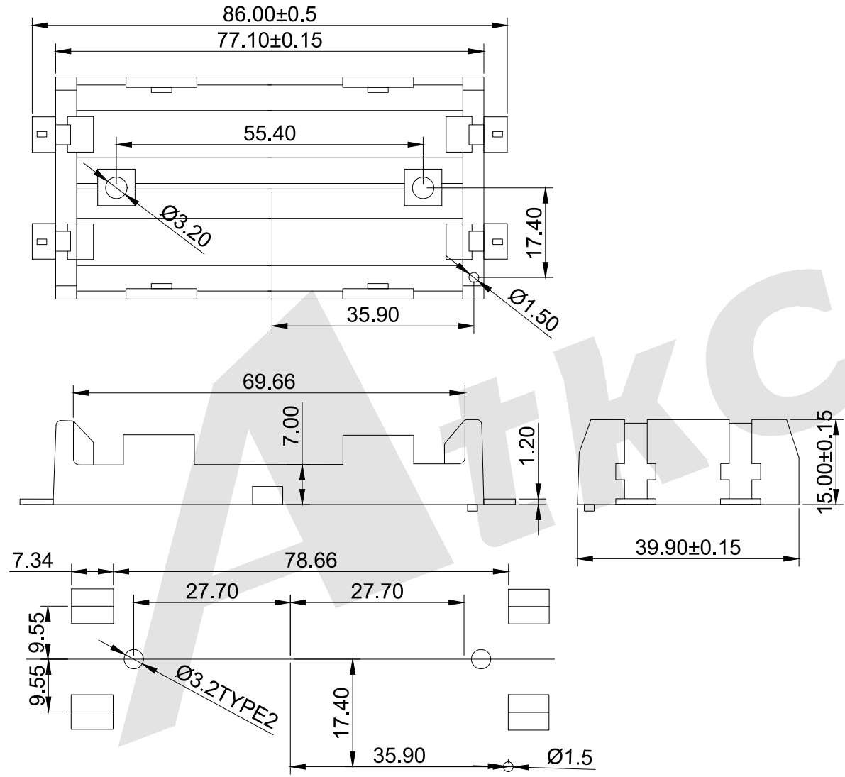
PCB LAYOUT
