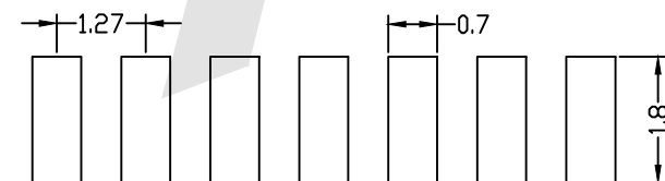
PCB LAYOUT
