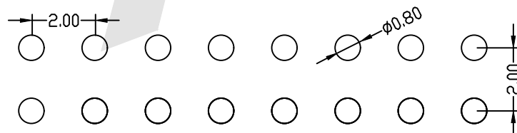
PCB LAYOUT
