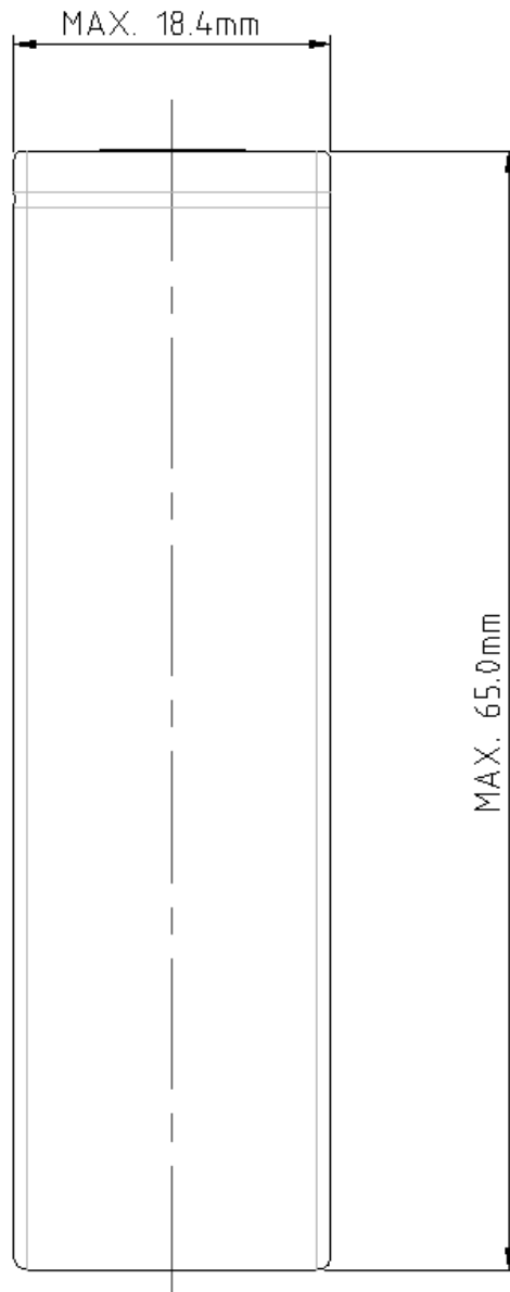
Fig.1. Outline Dimensions of ICR18650-26F
